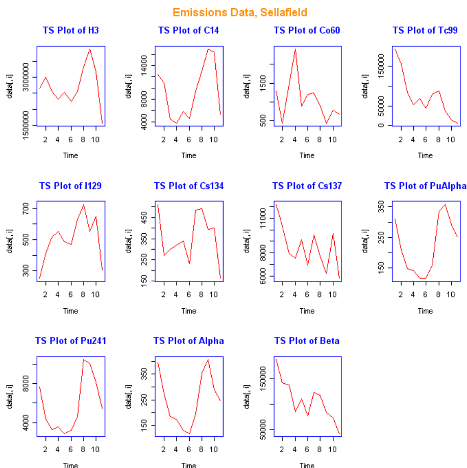
Figure 2A.1 Time Series (TS) Plots for Sellafield Discharges 1995-2005
