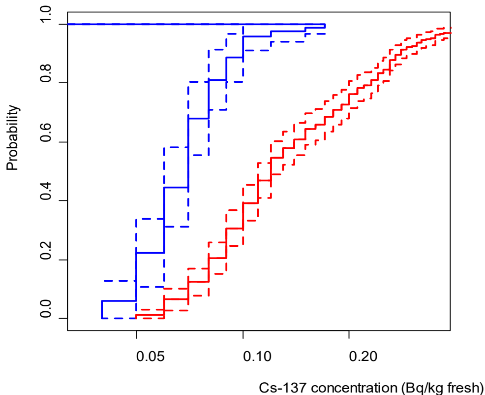
Figure 3: Empirical cumulative probability distribution functions estimates by Kaplan-Meier method (right and red: baseline; left and blue: assessment period). Dotted lines correspond to 95% confidence intervals on probability values. For the assessment period (left and blue), lower values are more probable.
