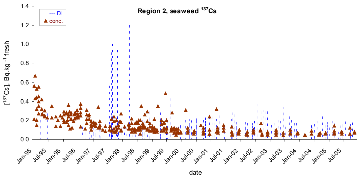
Figure 2: Time series measurements of ^{137}\text{Cs} concentrations ( \text{Bq.kg}^{-1} fresh) in seaweed from region 2 (triangle symbols). Non-detects values are represented by a vertical dotted line between zero and the DL value which means that the actual value lies within this interval.
