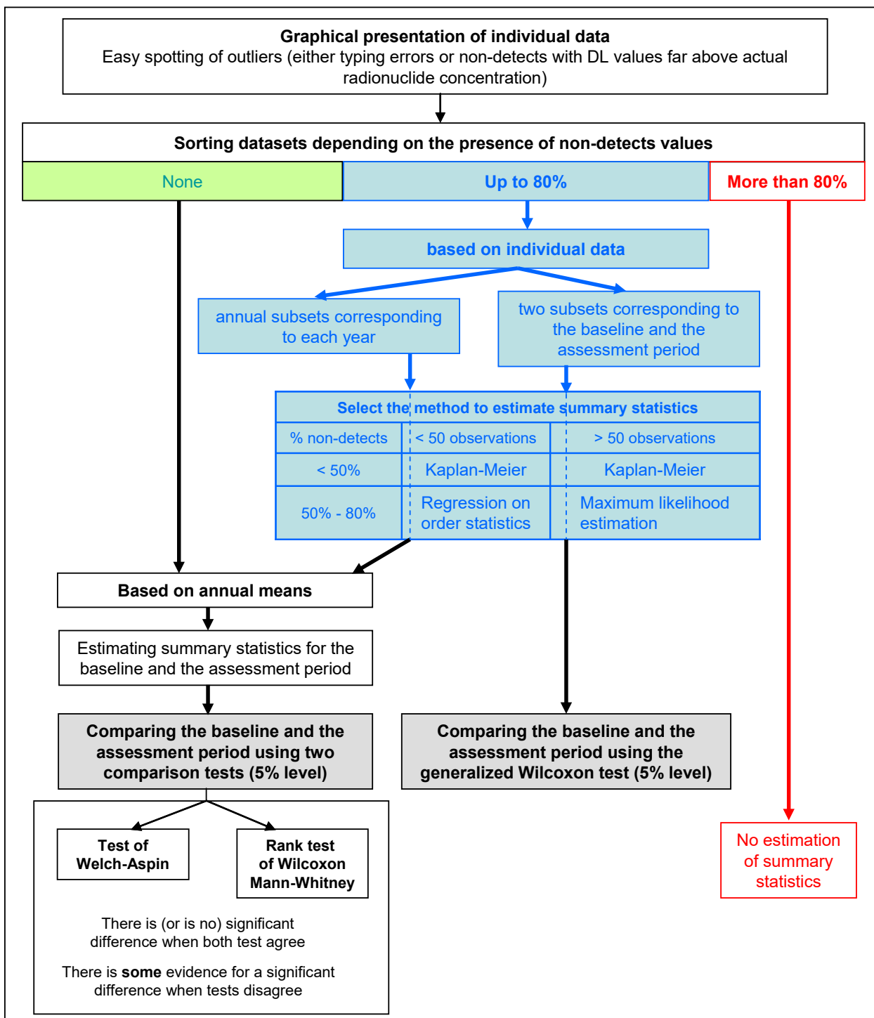
Figure 4 : Decision Flowchart depicting the general data processing for datasets.
