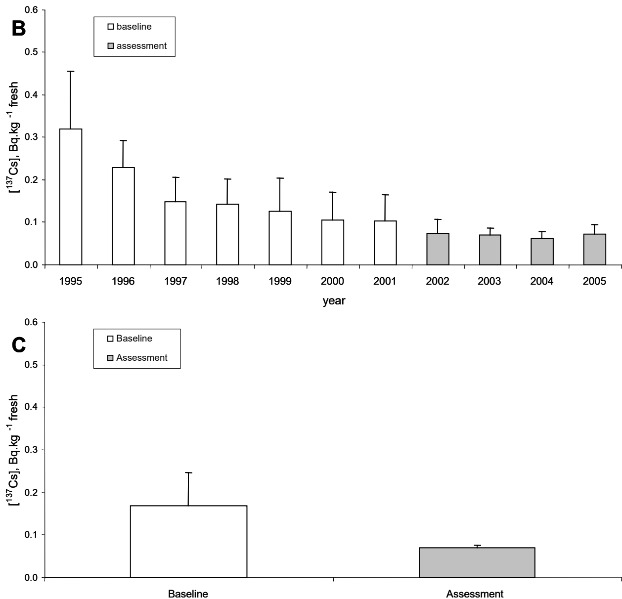
Figure 1: A: time series measurements of ^{137}\text{Cs} concentrations ( \text{Bq.kg}^{-1} \text{ fresh} ) in seaweed from region 2; B: Data provided by Contracting Parties as annual means; C: Baseline and Assessment period corresponding to the mean and standard deviation of annual means from [1995 – 2001] and [2002 - 2005], respectively.
