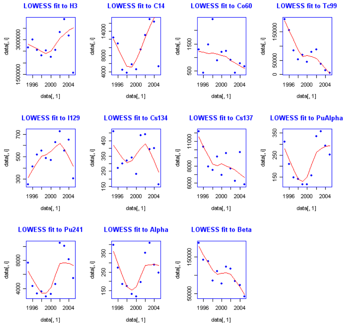
Figure 2A.5 Lowess fits to Sellafield Discharges data 1995-2005
