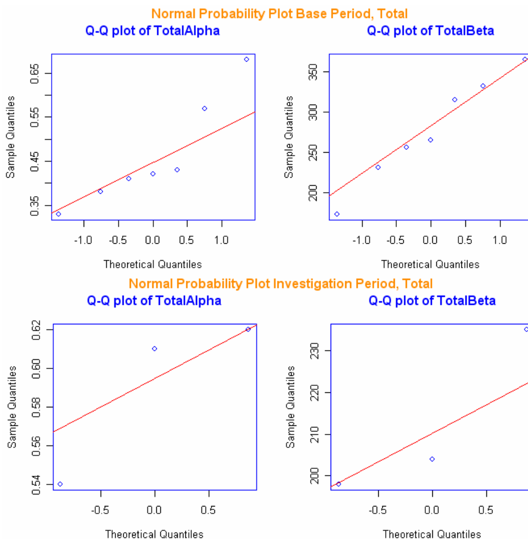
Normal Probability Plots for Overall Discharges 1995-2001 and 2002-2004
