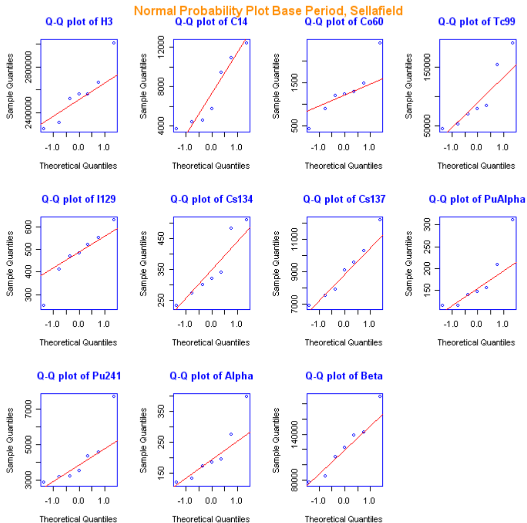
Figure 2A.2 Normal Probability Plots for Sellafield Discharges: baseline period 1995-2001
