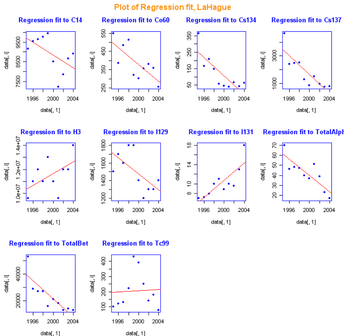
Figure 2B.4 Linear Regression fits to La Hague Discharges data 1995-2004
