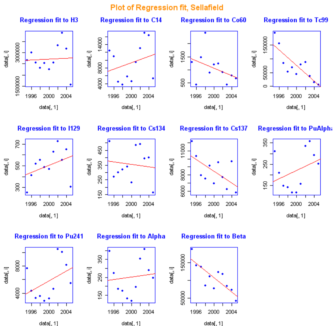
Figure 2A.4 Linear Regression fits to Sellafield Discharge data 1995-2005
