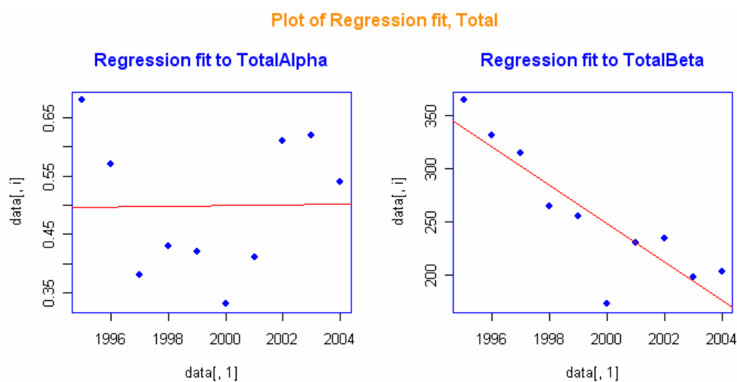
Linear Regression fits to Overall Discharges data 1995-2004
