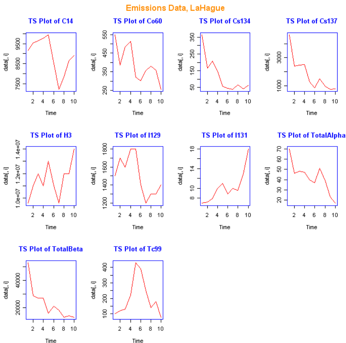
Figure 2B.1 Time Series Plots for La Hague Discharges 1995-2004
