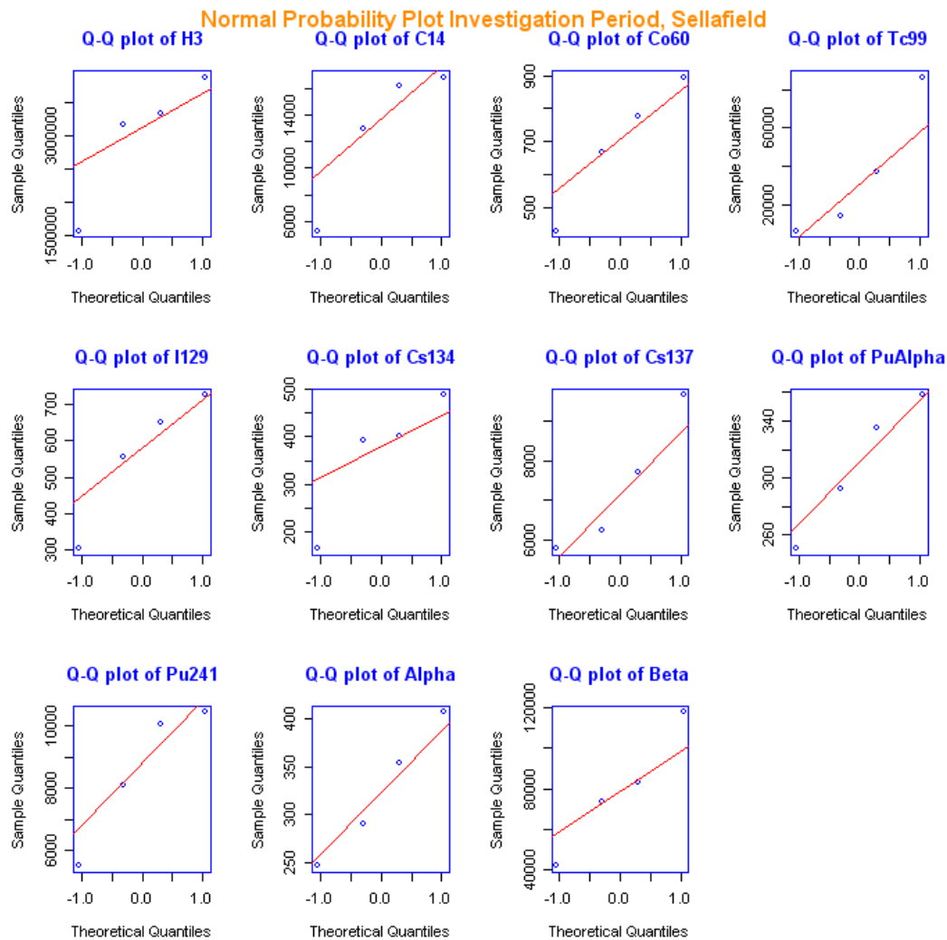
Figure 2A.3 Normal Probability Plots for Sellafield Discharges: assessment period 2002-2005
