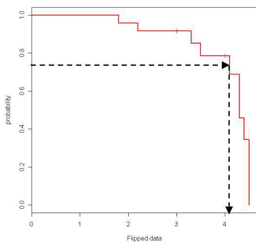
Figure 1.1: Survival probability function S of the multiply-censored flipped Oahu data.
