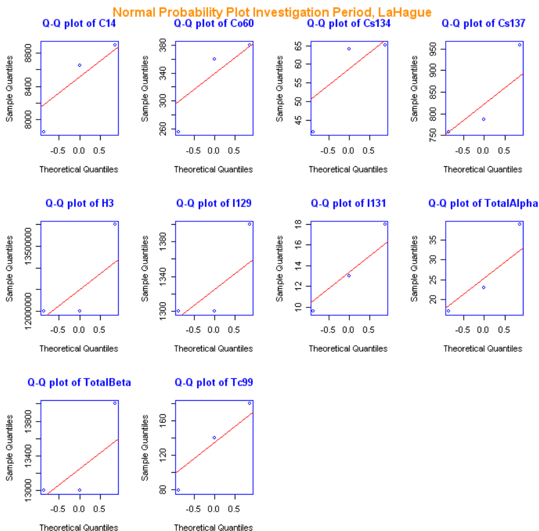
Figure 2B.3 Normal Probability Plots for La Hague discharges 2002-2004
