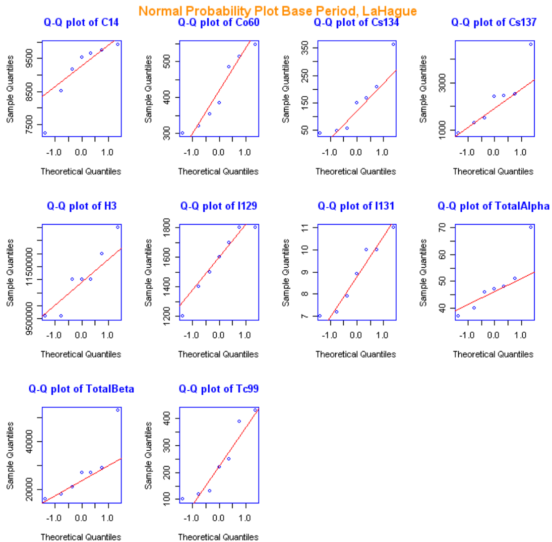
Figure 2B.2 Normal Probability Plots for La Hague discharges 1995-2001
