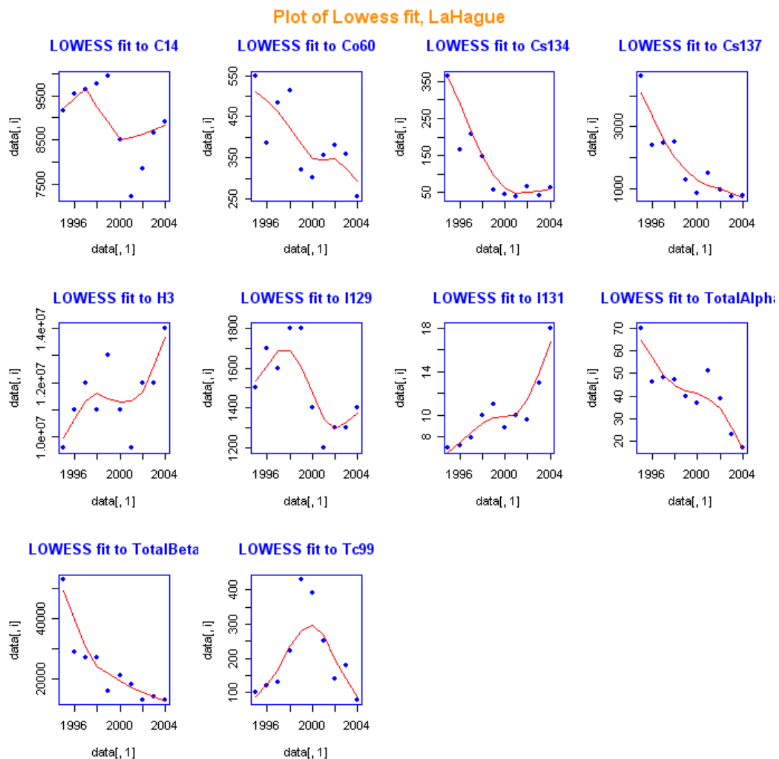
Figure 2A.5 Lowess fits to La Hague Discharges data 1995-2004
