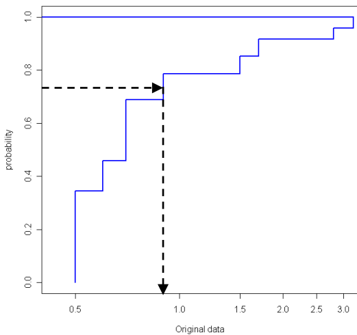
Figure 1.2: Empirical cumulative distribution function of the multiply-censored Oahu original data.
