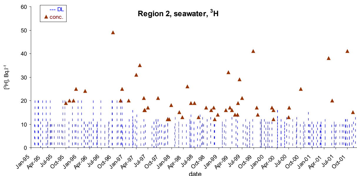
Figure 6: Time series measurements of ^3\text{H} concentrations ( \text{Bq.L}^{-1} ) in seawater from region 2 (triangle symbols). Non-detects values are represented by a vertical dotted line between zero and the DL value which means that the actual value lies within this interval.
