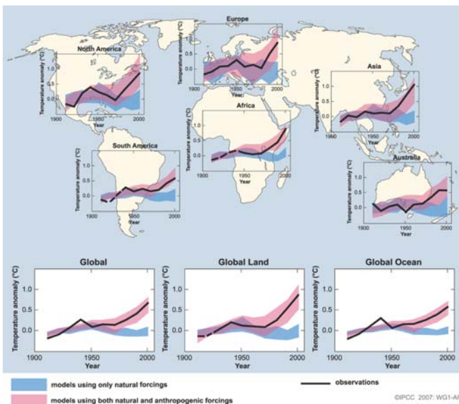
2 3 4 5 6 Figure 1.2 IPCC figure of time series 7 showing observed 20th century climate 8 (black) versus climate models with (pink) 9 and without (blue) anthropogenic GHG. 10 [Reproduced from IPCC AR4 WG1 Chp 9 11 FAQ 9.2] (IPCC, 2007a) 12
