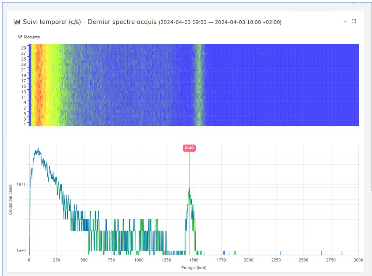
Figure: Gammaspec water probe interface - waterfall view (above) – spectrum view (below)
